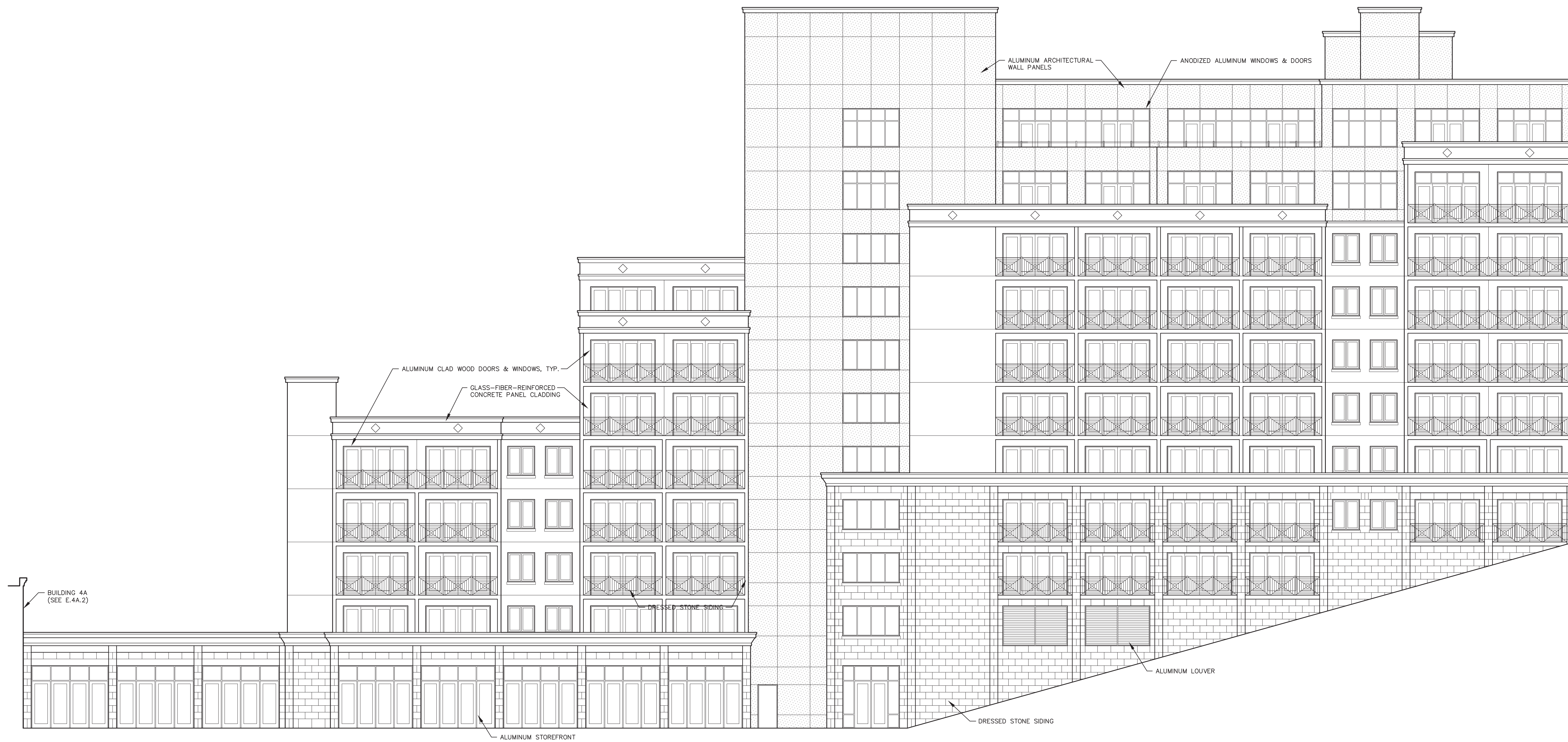
NORTH WING - NORTH ELEVATION
