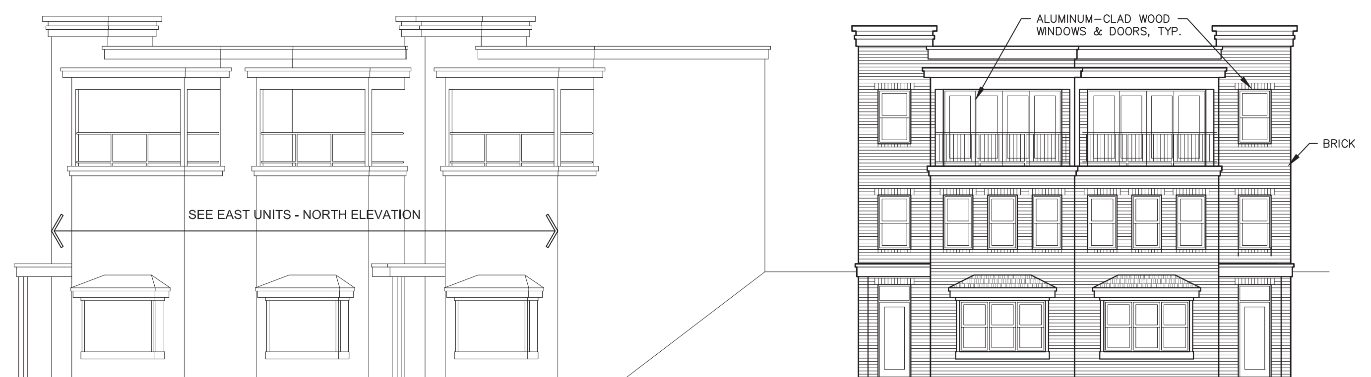
WEST UNITS - NORTH ELEVATION
