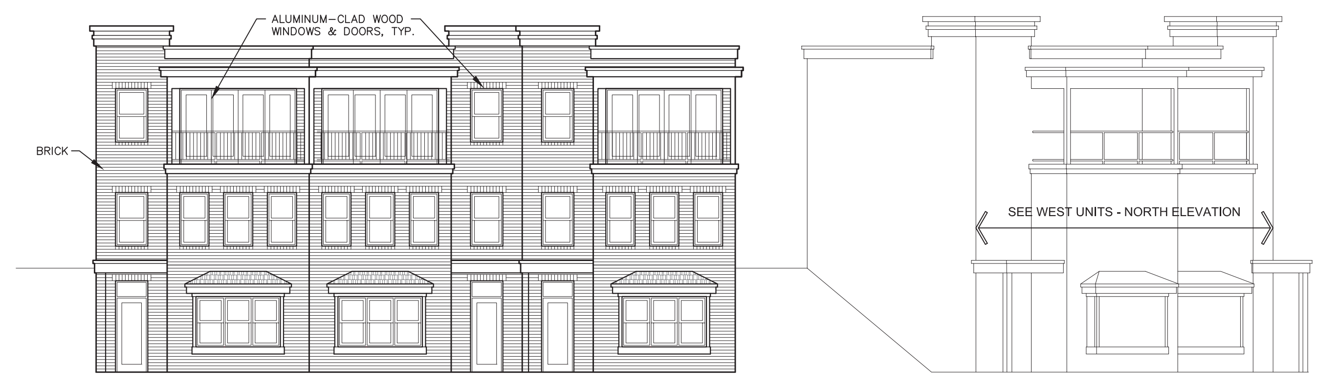
EAST UNITS - NORTHEAST ELEVATION
